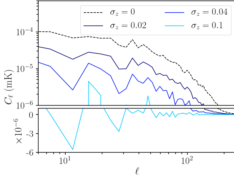
Figure 4.12: Cross-correlation between HI intensity maps with FASTICA reconstruction and an optical survey using GAEA at z = 0.25 with \Delta z = 0.02 bin width. I degrade the constraints on the optical galaxy redshifts by increasing the redshift error \sigma_z shown by going from dark to lighter blue. In other words I go from cross-correlating intensity maps with a spectroscopic-like ( \sigma_z \sim 0 ) survey, to a photometric-like survey where there is significant uncertainty on the optical galaxy redshifts. This strongly affects the measured cross-correlation power spectrum. Plot includes a hybrid log-linear y -axis to fully demonstrate the degradation in power.
