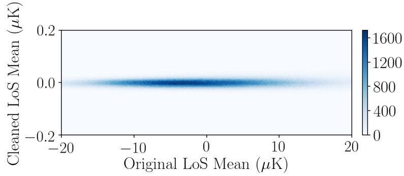
Figure 4.14: The mean \delta T temperatures along the line-of-sight (LoS) for the original HI intensity map against one with which has undergone a FASTICA foreground clean. This is shown for all available LoS in the GAEA simulation which for f_{\text{sky}} = 0.5 and n_{\text{side}} = 512 equates to over 1.5 million pixels (or LoS). The plot shows how FASTICA essentially removes any non-zero LoS mean present in the original HI signal and collapses it to zero.
