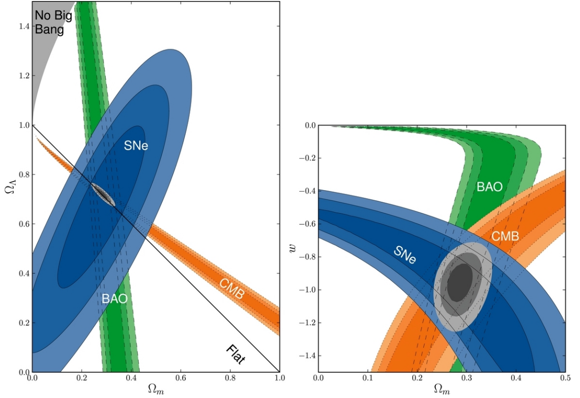
Figure 1.4: Constraints on cosmological parameters from three combined probes; Supernovae (SNe), Cosmic Microwave Background (CMB) and Baryon Acoustic Oscillations (BAO). Produced by the Supernova Cosmology Project [203]. 68.3%, 95.4%, and 99.7% confidence regions shown.
