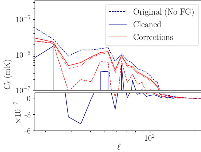
Figure 4.17: Cross-correlation angular power spectrum for the MICE simulation at redshift of z = 1.075 with \Delta z = 0.05 bin width and like Figure 4.13 I have used the DES-like photometric redshifts available in MICE. Again the impact from foregrounds is visible in the difference between the blue dashed line and blue solid line. However, the effectiveness of the corrective techniques that I outlined in Section 4.5.2, shown by the red lines, is encouraging. The dashed red line is for the LoS mean correction, the dotted red line represents the extended- z correction and the red solid line represents both corrections applied. Produced using bandpowers with 6 multipoles per bin for clarity.
