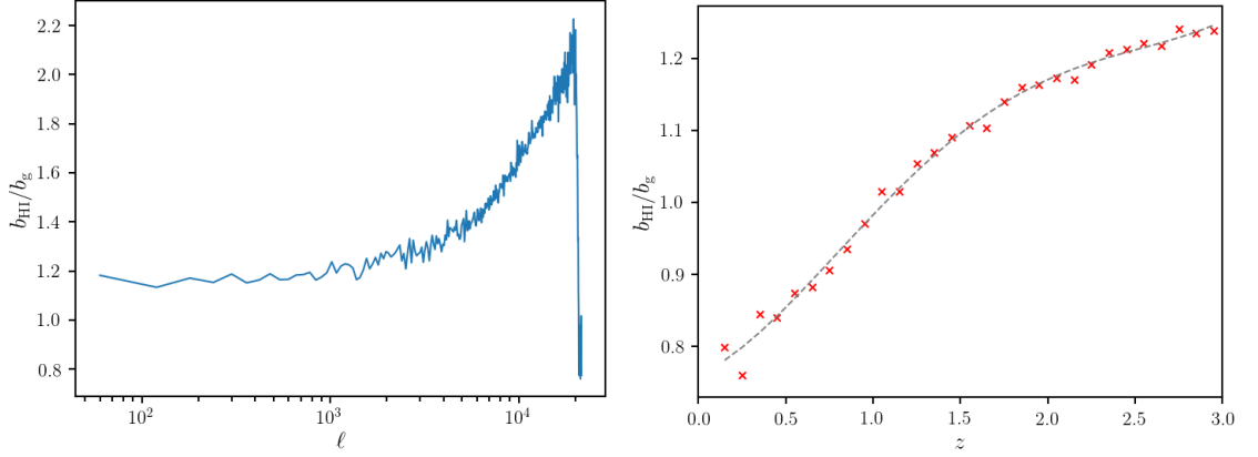
Figure 3.3: [Left] The bias ratio b_{\text{HI}}/b_g as a function of angular scale at redshift z = 2 . This ratio is only constant on the largest scales so we therefore choose to measure this bias at scales with \ell < 10^3 . [Right] The bias ratio b_{\text{HI}}/b_g as per equation (3.24) in each redshift bin with the grey dashed line showing a polynomial fit to the data points. As expected, the bias ratio that I use in our estimator evolves with redshift.
