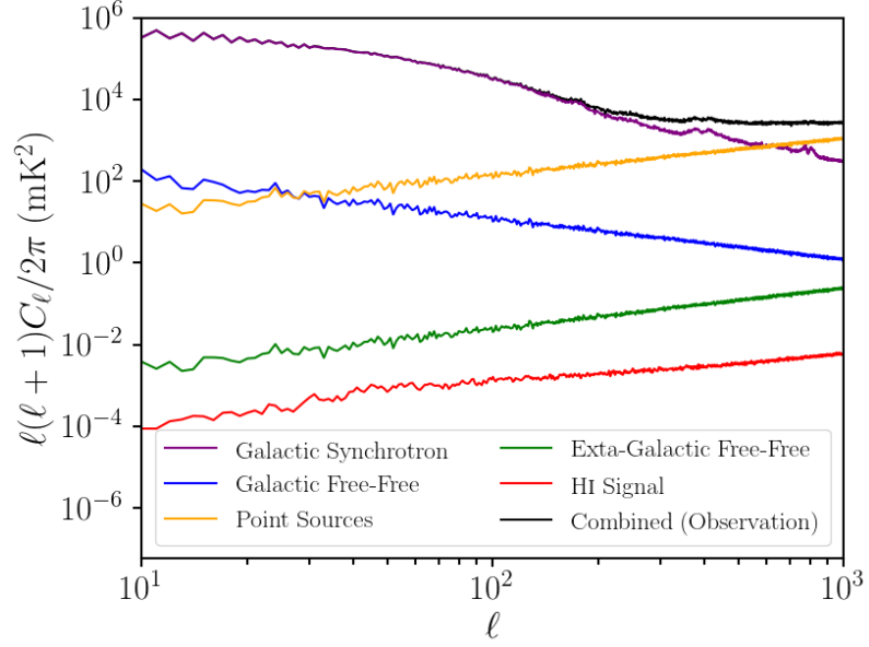
Figure 4.5: Angular power spectra for all the different simulated foregrounds, and the HI cosmological signal produced using the GAFA catalogue. The black solid line represents the combined signal from all foregrounds and the HI cosmological signal. All are at a frequency of 1136MHz ( z = 0.25 ) and noise free with no beam effects added.
