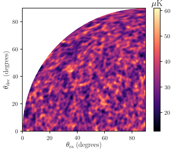
Figure 3.9: Large sky HI intensity map using MICE catalogue galaxies with halo masses converted into predicted HI masses. Since this is now a much larger patch of sky, we can no longer make the flat-sky approximation, and therefore I use a HEALPix projection for the map. This particular example is a slice taken at 0.60 < z < 0.65 with \theta_{\text{FWHM}} \approx 1.3^\circ .
