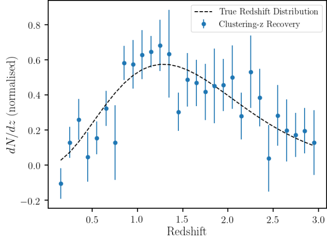
Figure 3.8: Increasing the beam size to \theta_{\text{FWHM}} = 16' for our \text{S}^3\text{-SAX} sample, which is equivalent to reducing the resolution of our experiment, causes errors to increase as predicted by equation (3.27).
