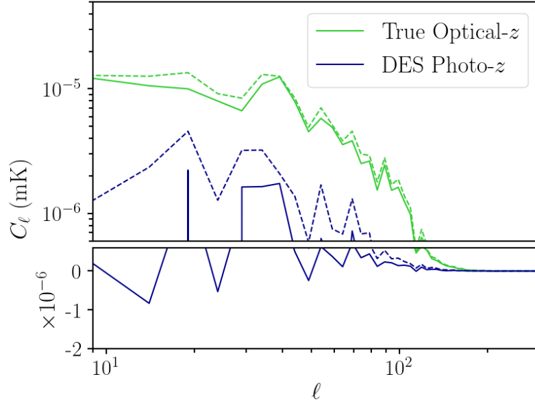
Figure 4.13: Cross-correlation between HI intensity maps with MICE optical galaxies. Dashed lines show the cases without HI foregrounds, solid lines show the impact of including them. I use the DES-like photometric redshifts available in MICE for the photo- z forecasts shown in blue and compare these with using ideal true redshifts (green). While a drop in signal is inevitable when using less constrained redshifts, including the effects of HI foregrounds (solid lines) degrades the signal further in the photo- z case. These tests have been performed at redshift z = 0.725 with \Delta z = 0.05 bin width.
